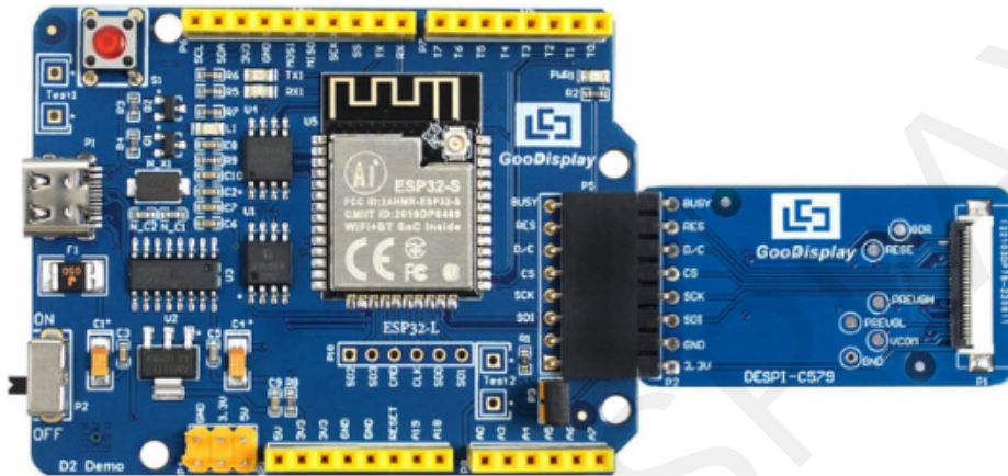
Figure 3 : Connection between ESP32-L for EPD and DESPI-C579
